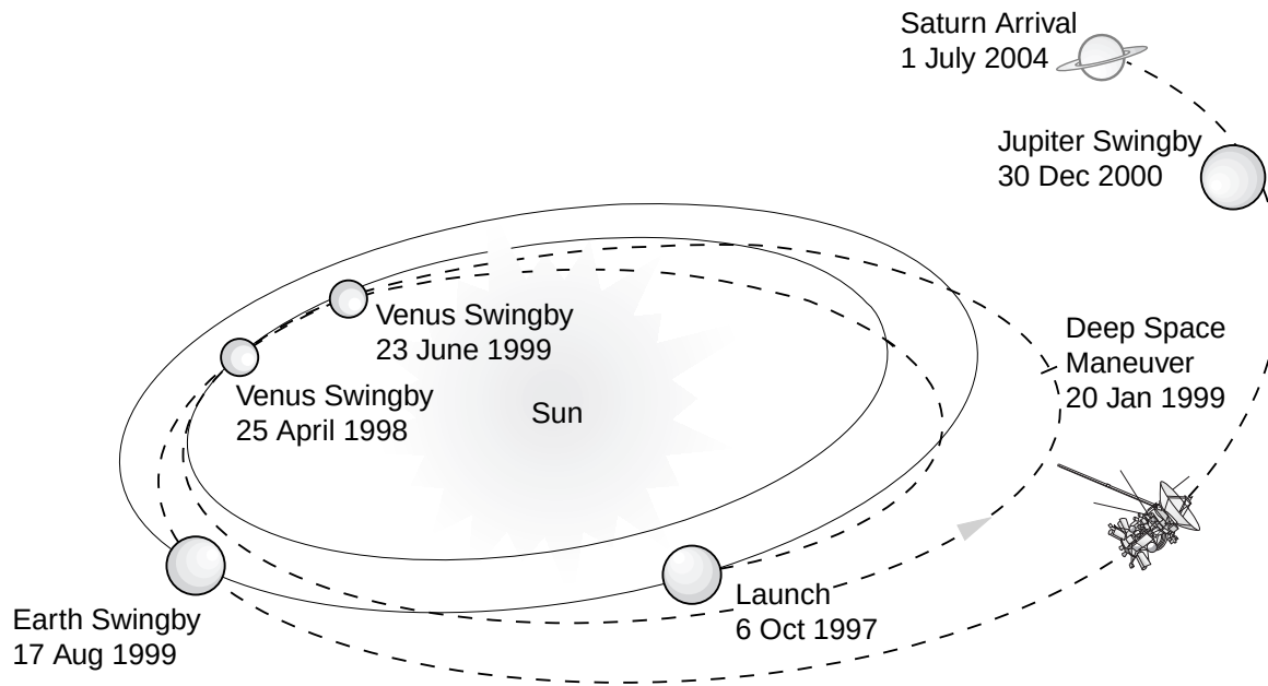
Interplanetary Trajectory
