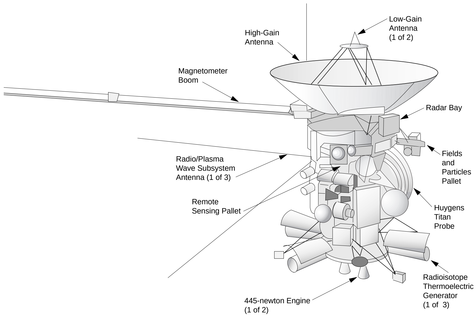
Cassini spacecraft
