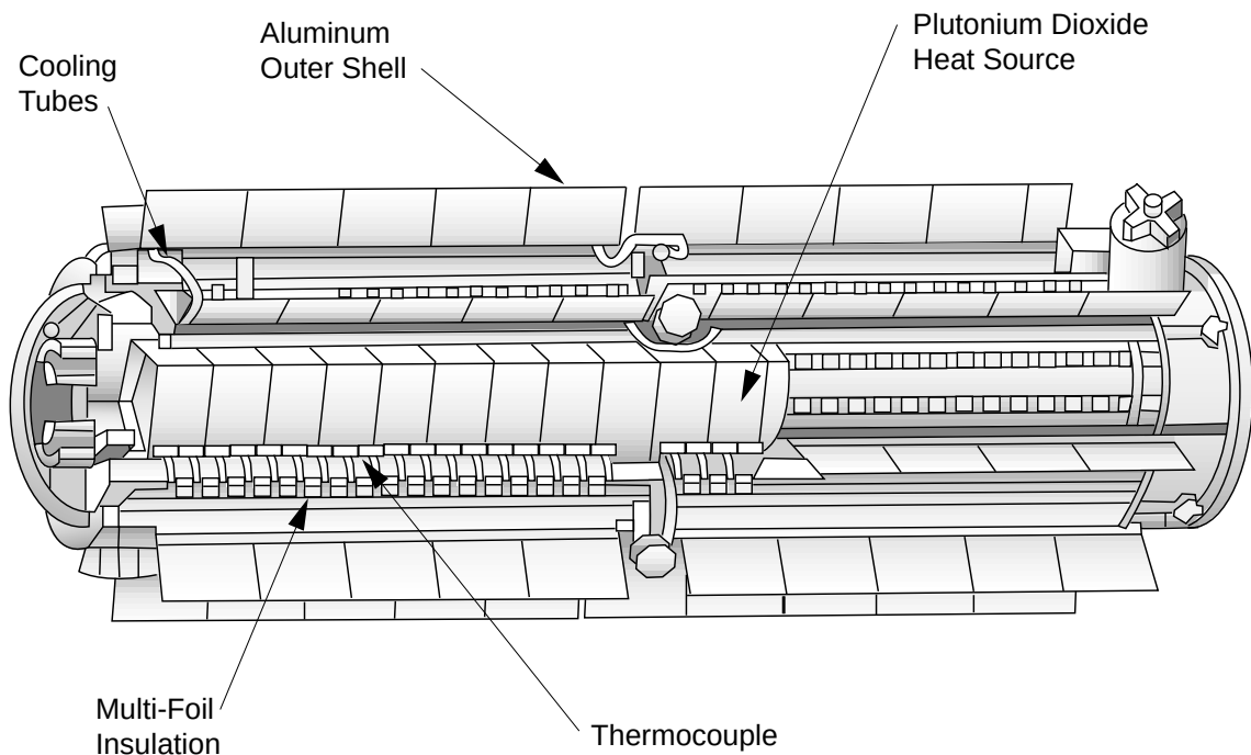
Radioisotope thermoelectric generator (RTG)
